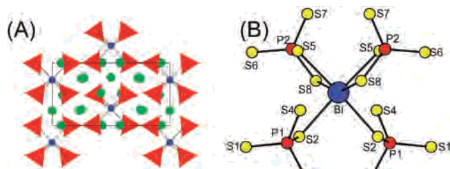
Figure 8. (A) View down [010] of III and (B) a view of an individual molecule of [\text{Bi}(\text{PS}_4)]_9^- .
